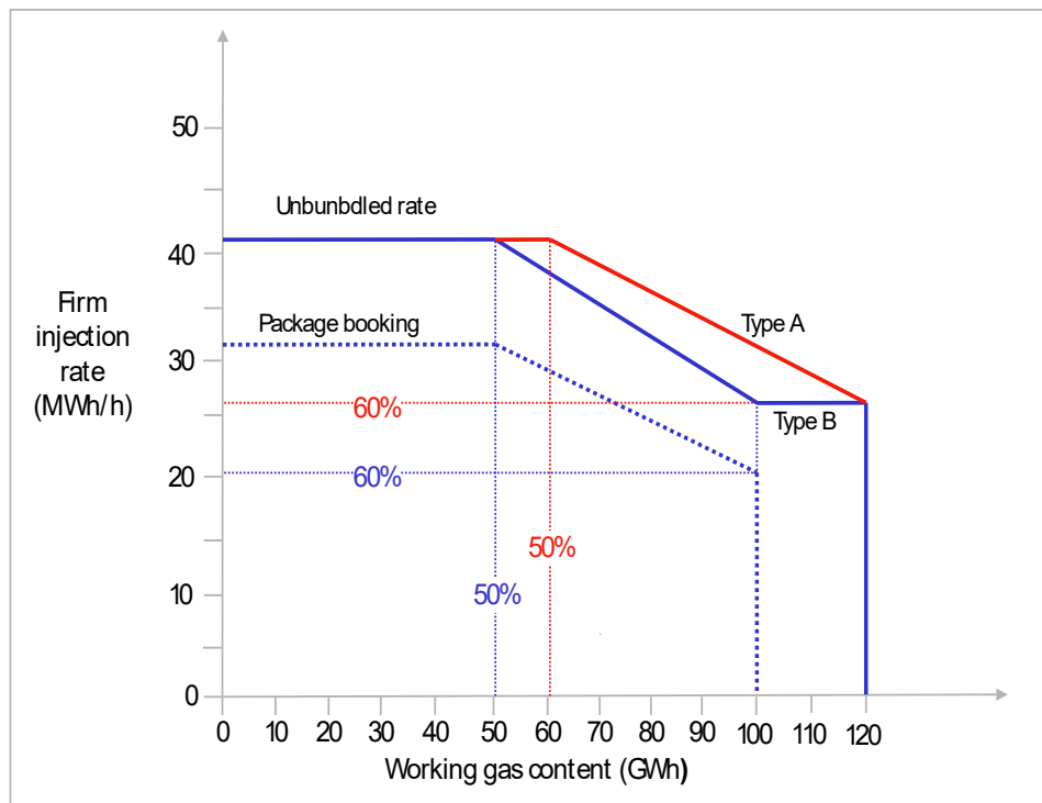
Figure 2: Injection rate curve for a firm storage capacity
